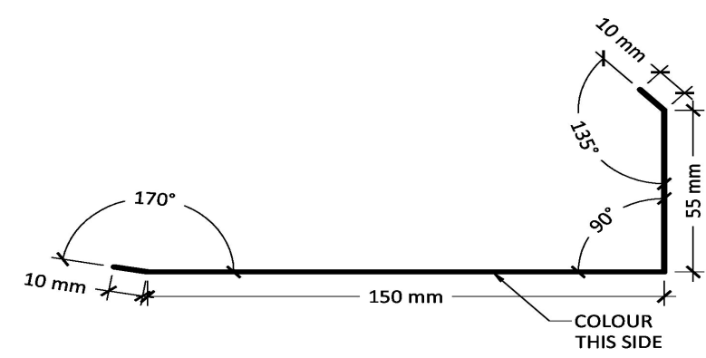
Corner Flashing A-RDJAMB-I-A-0
