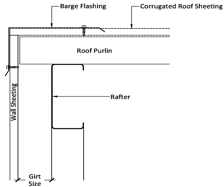
Barge Flashing - A-BARGE-1 - Sheeting Gable
